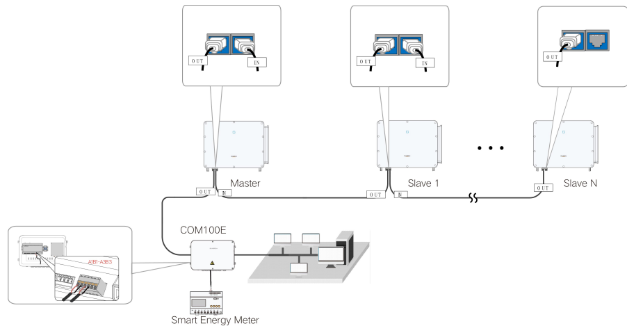
Figura 5-6 Multi-inverter Communication System 【RS485_1 interface (RJ45)】
