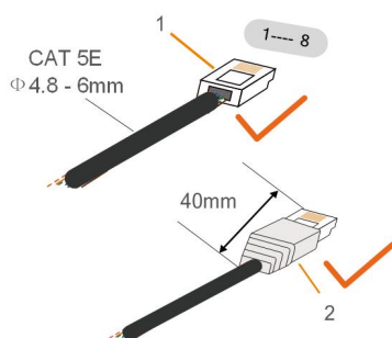
1: Plugue RJ45
