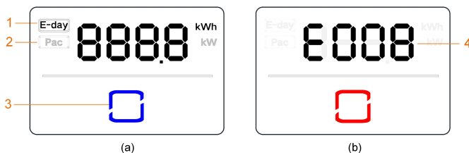
Figura 2-4 Painel LED
